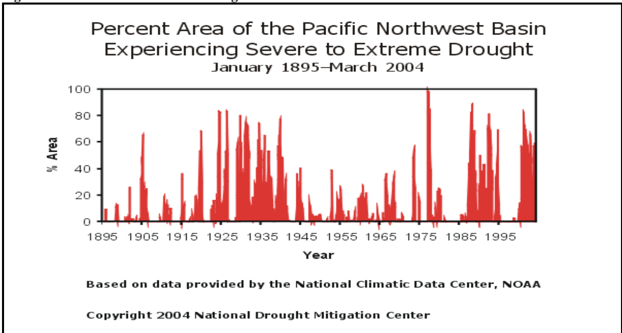
Figure 4.M2-2 % Area of Basin in Drought Conditions Since 1895 5
