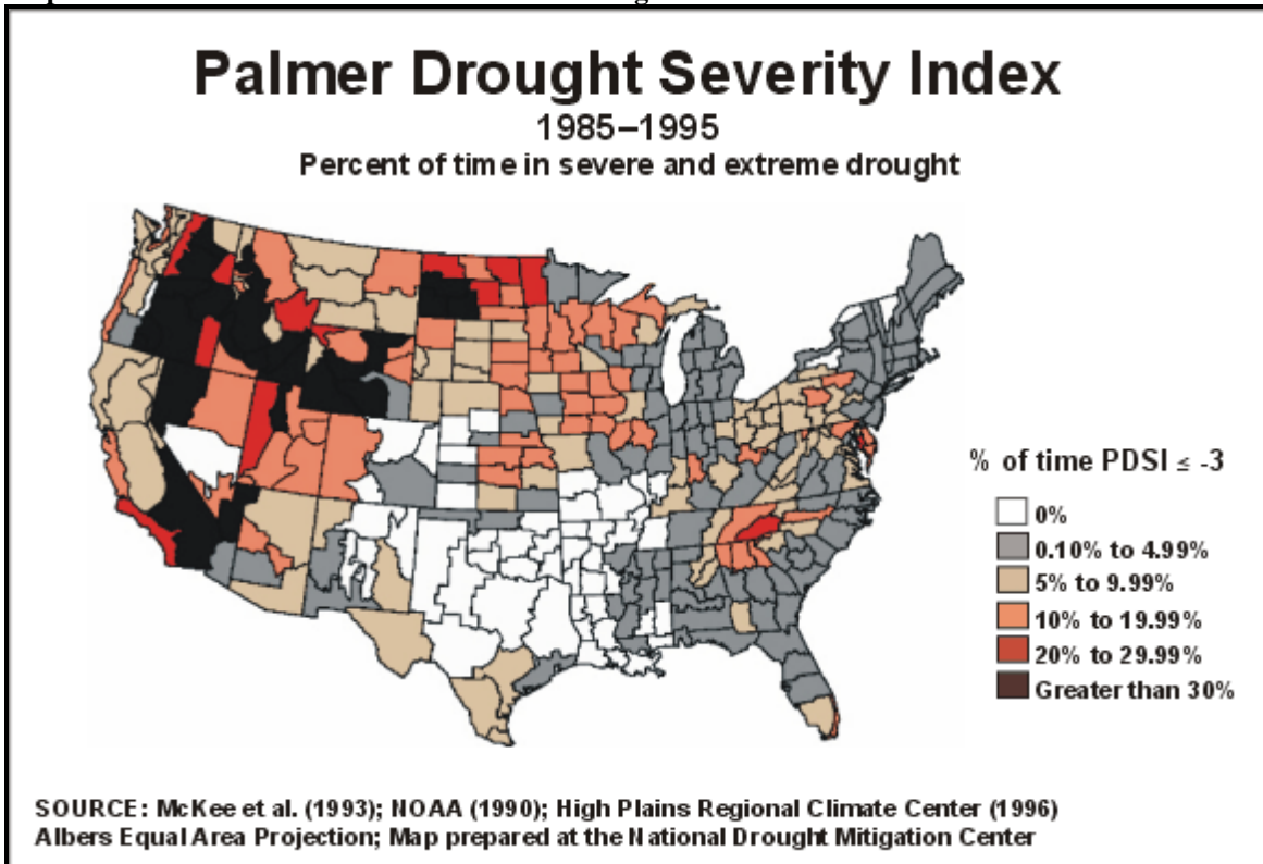
Map 4.M2-3 % of Time in Severe to Extreme Drought 1985-1995
