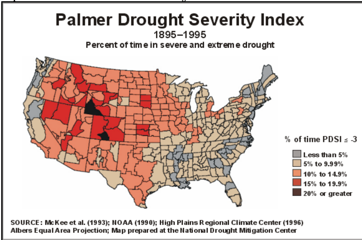
Map 4.M2-2 % of Time in Severe to Extreme Drought: 1895-1995
