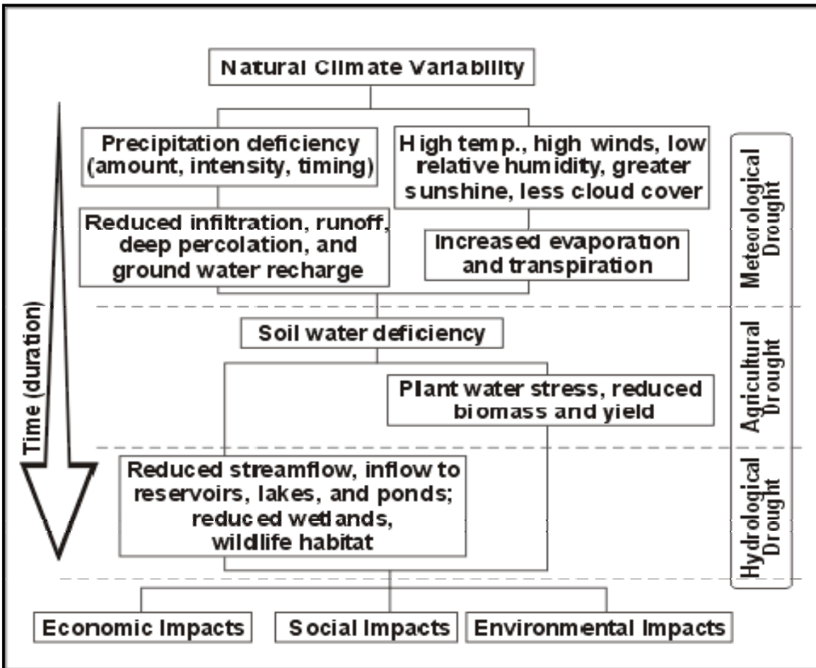
Figure 4.M2-1 Sequence of Drought Impacts 1
